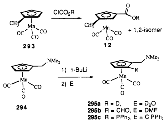
Scheme 70 93,40
