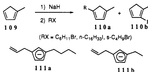
Scheme 24 47,30
