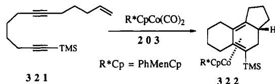
Scheme 80 4
