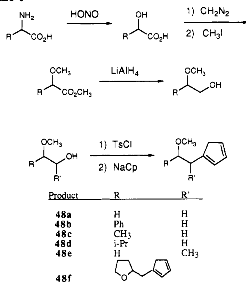
Scheme 9 29
