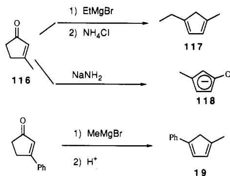
Scheme 26 49,50,18
