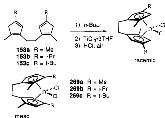
Scheme 62 67
