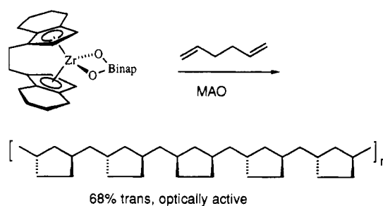
Scheme 84 122
