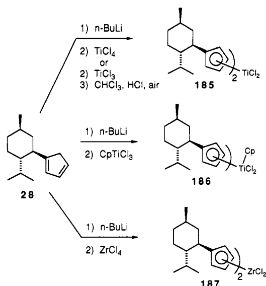
Scheme 45 3,8,26
