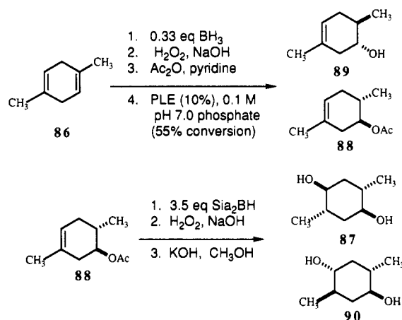
Scheme 19 9
