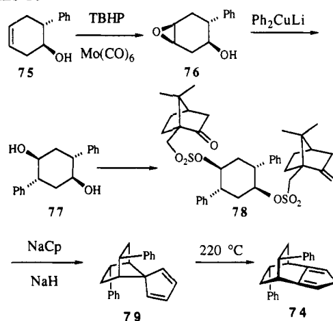
Scheme 16 40
