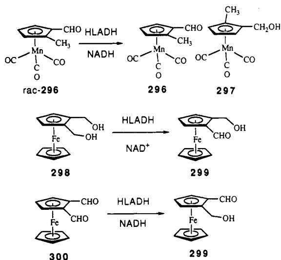
Scheme 70 93,40
