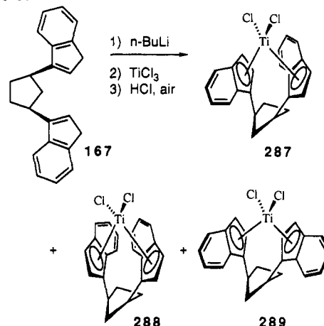
Scheme 67 67
