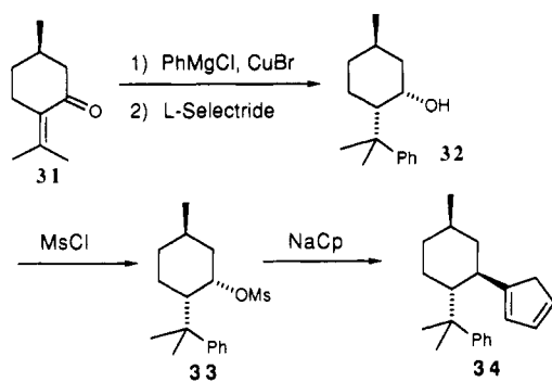
Scheme 7 25
