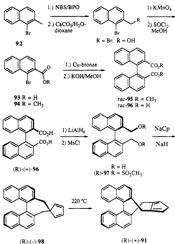
Scheme 20 42
