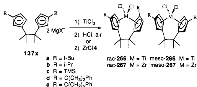
Scheme 59 62,63
