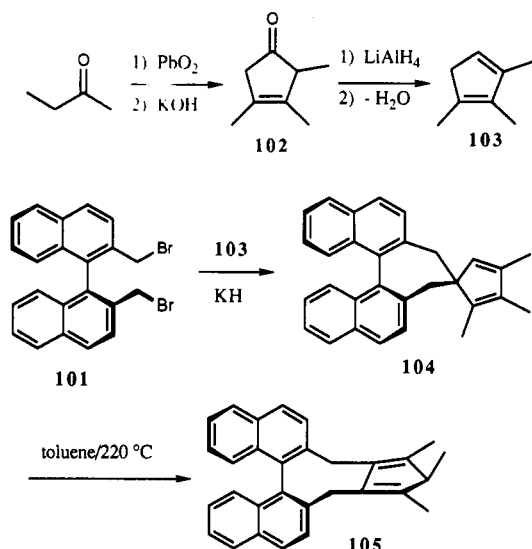
Scheme 23 46
