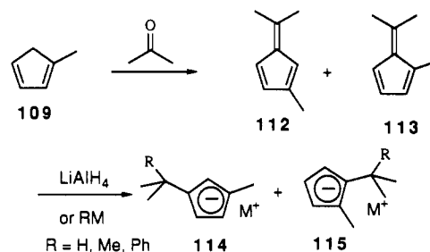
Scheme 26 49,50,18
