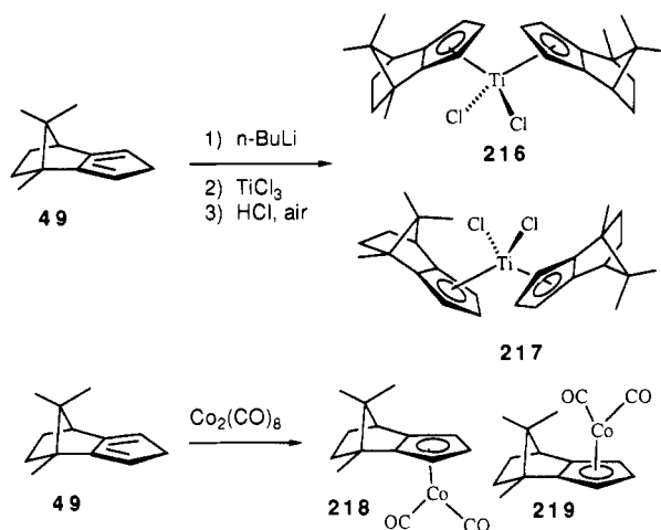
Scheme 49 35,36
