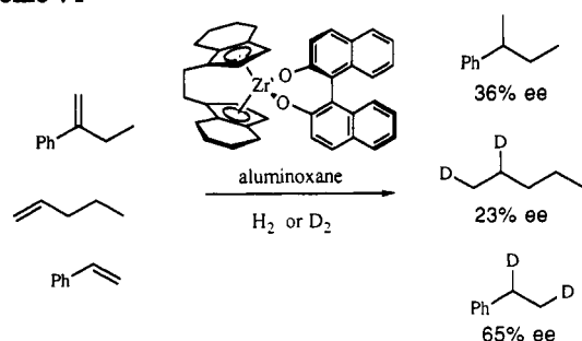
Scheme 74 104
