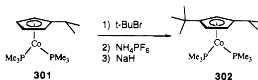
Scheme 72 96-99
