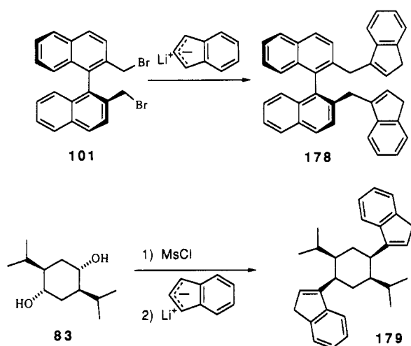
Scheme 43 11,38
