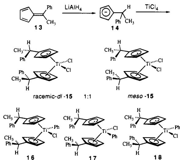
Scheme 2 18
