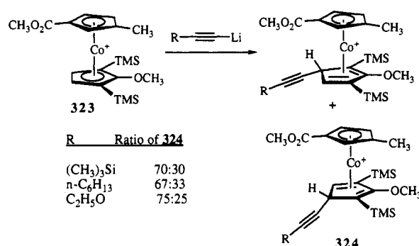
Scheme 80 4
