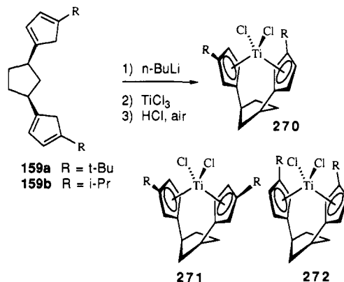
Scheme 62 67
