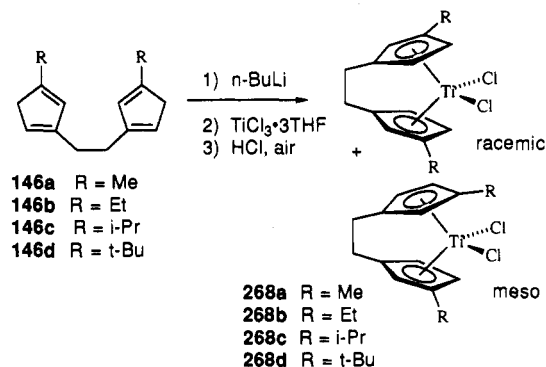
Scheme 60 65
