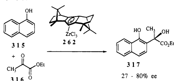
Scheme 78 111
