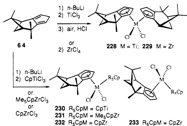
Scheme 51 86,36
