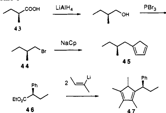
Scheme 9 29
