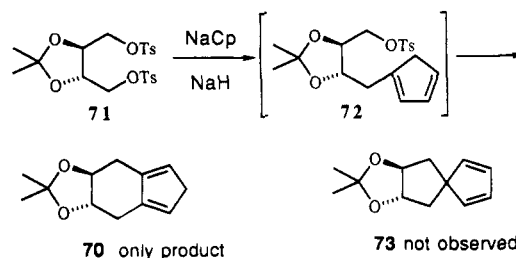
Scheme 16 40
