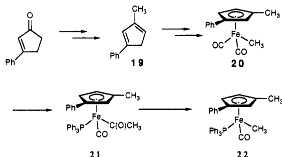
Scheme 2 18
