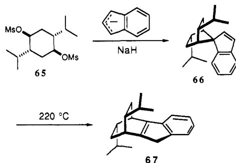
Scheme 14 39
