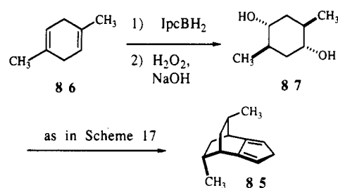
Scheme 19 9
