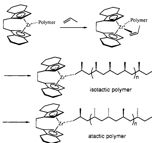
Scheme 84 122
