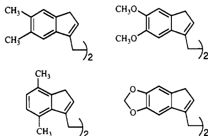
Figure 4. Substituted bis(indenes). 75
